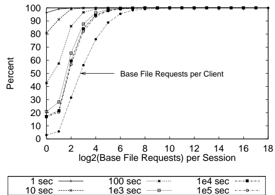
Figure 6 Analysis of Base Files Requested Per Session
