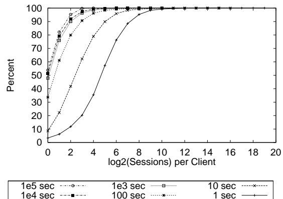
Figure 4 Analysis of the Number of Sessions Per Client
