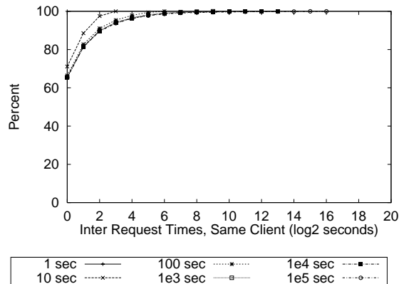
Figure 8 Inter-Request Times in Individual User Sessions
