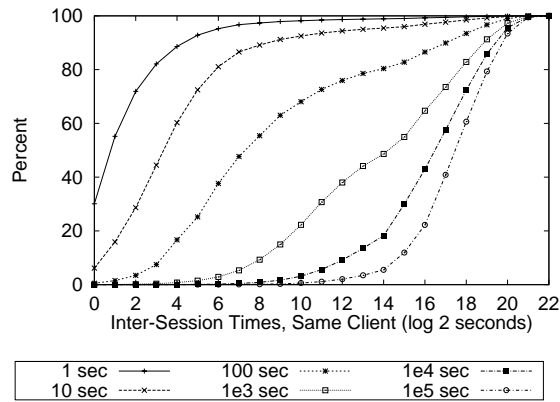
Figure 7 Analysis of Inter-Session Times
