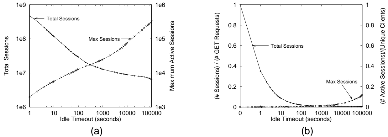
Figure 2 Effect of Timeout Values on Total Number of Sessions
