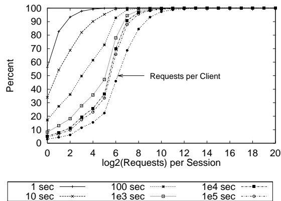
Figure 5 Analysis of Requests per Session
