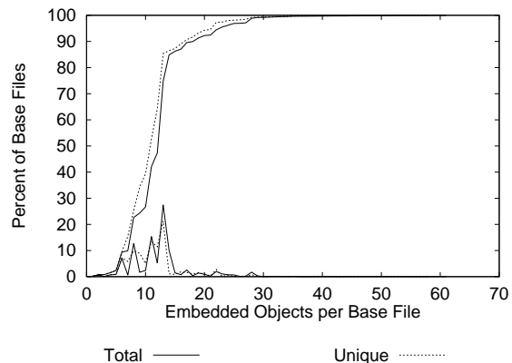
Figure 1 Analysis of Embedded Files per Base File
