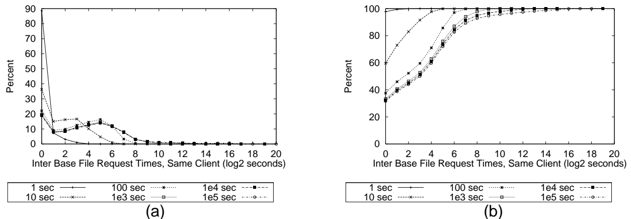
Figure 9 Analysis of Inter-Request Times for Base Files: (a) Frequency; (b) Cumulative Frequency
