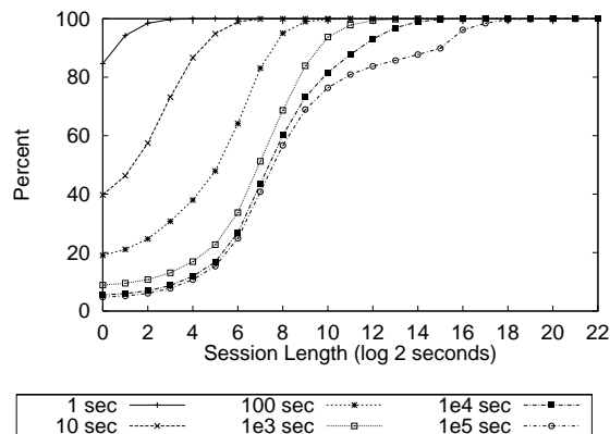
Figure 3 Analysis of Session Lengths
