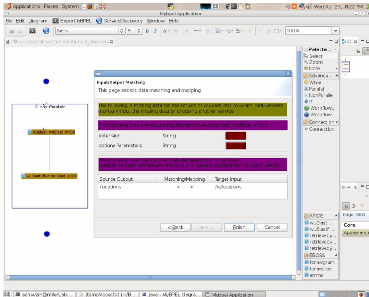
Figure3: WS Composition Editor with Wizard
