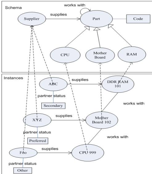
Figure 6: Supply Chain Domain Ontology
