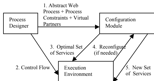
Figure 1: Architecture Overview
