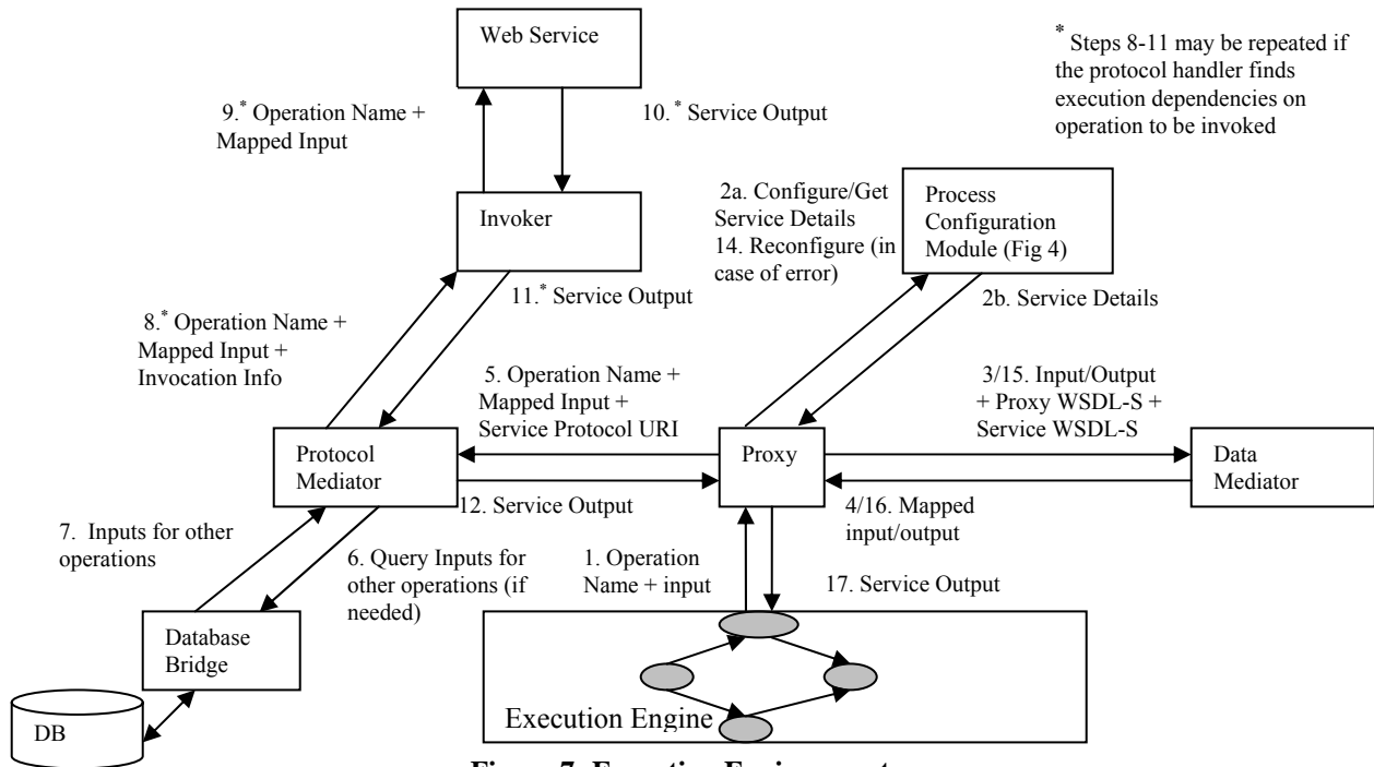
Figure 7: Execution Environment
