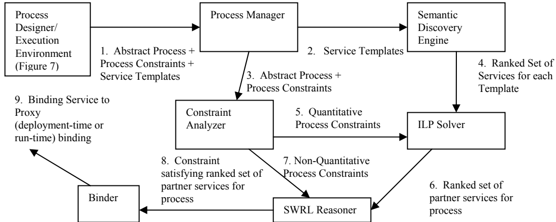
Figure 4: Process Configuration Module
