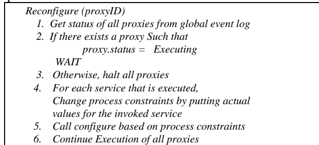
Figure 10: Algorithm for Reconfiguration
