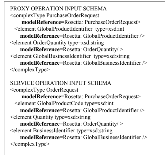
Figure 8: Proxy and Service Input Schemas
