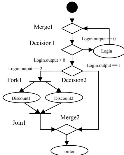
Figure 9: Example of an Interaction Protocol
