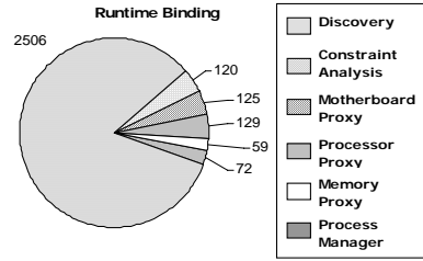
Figure 12: Component based time consumption during runtime binding.
