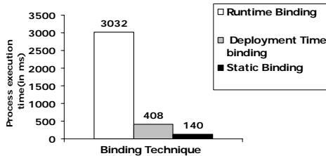
Figure 11: Comparison of execution times of different process composition approaches
