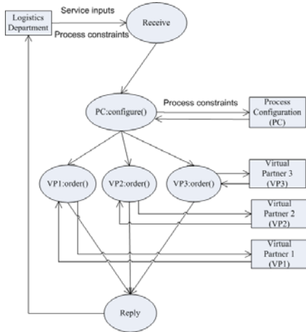
Figure 2: Abstract Web Process with Three Virtual Partners
