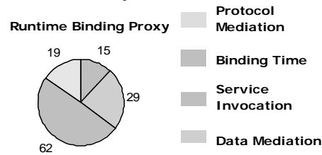
Figure 13: Breakdown of components invoked by execution environment during service invocation
