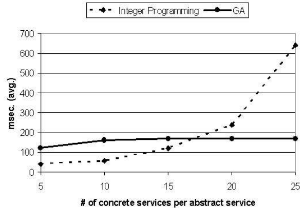
Figure 4: Comparison between Integer Programming and GAs
