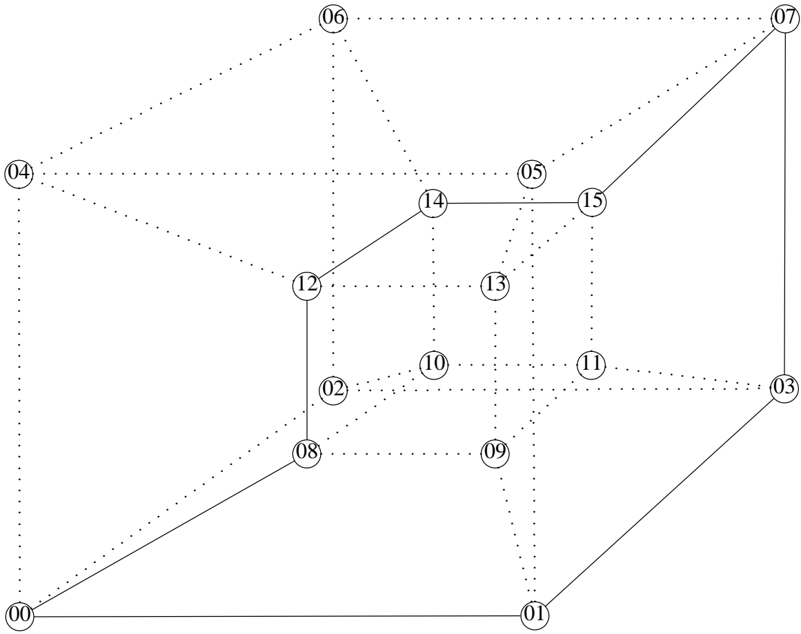
4-D Hypercube
