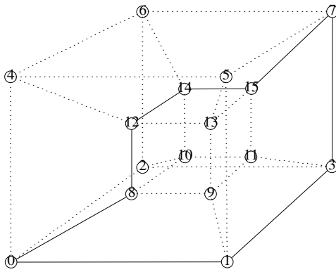
Figure 5. 4-D Hypercube
