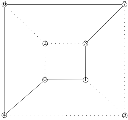
Figure 4. 3-D Hypercube
